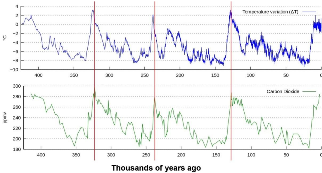
Fig. 2. From [11]. Temperature and carbon dioxide data from the Vostok ice-core [15-17]. Note that temperature rises before carbon dioxide, not vice versa. This figure shows compelling evidence that temperature rise results in a subsequent increase in atmospheric carbon dioxide content, in striking contradiction to the IPCC model-driven assumption that CO 2 causes global temperature increases. The rise or fall of CO 2 follows the increase or decline of Earth's variable heat, absorbed from above and produced from below
